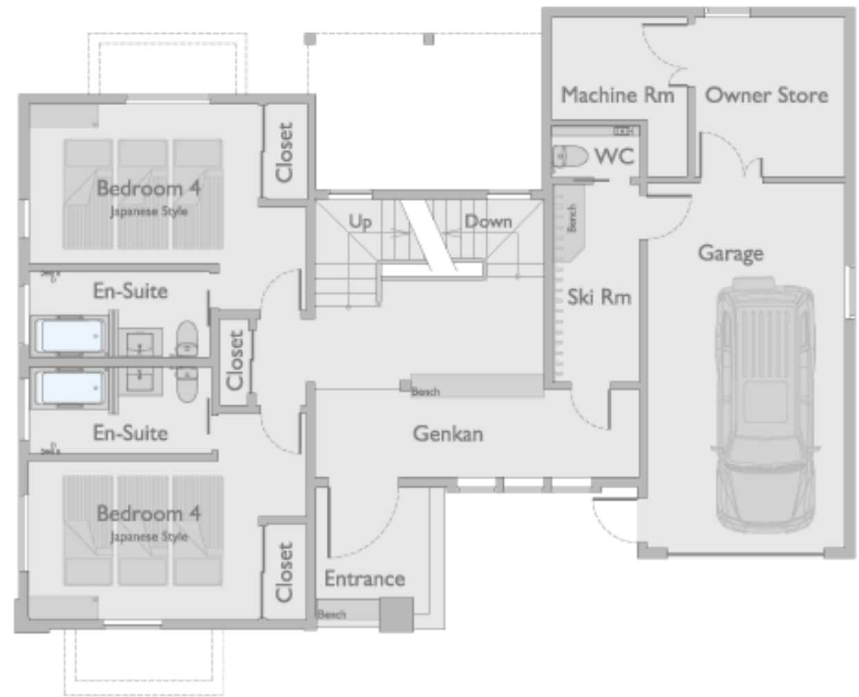
Middle Floor Plan
